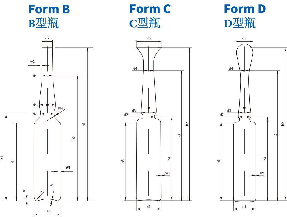
Ampoules specification (UNIT:mm) ISO 9187-1:2000 安瓿瓶的规格尺寸
