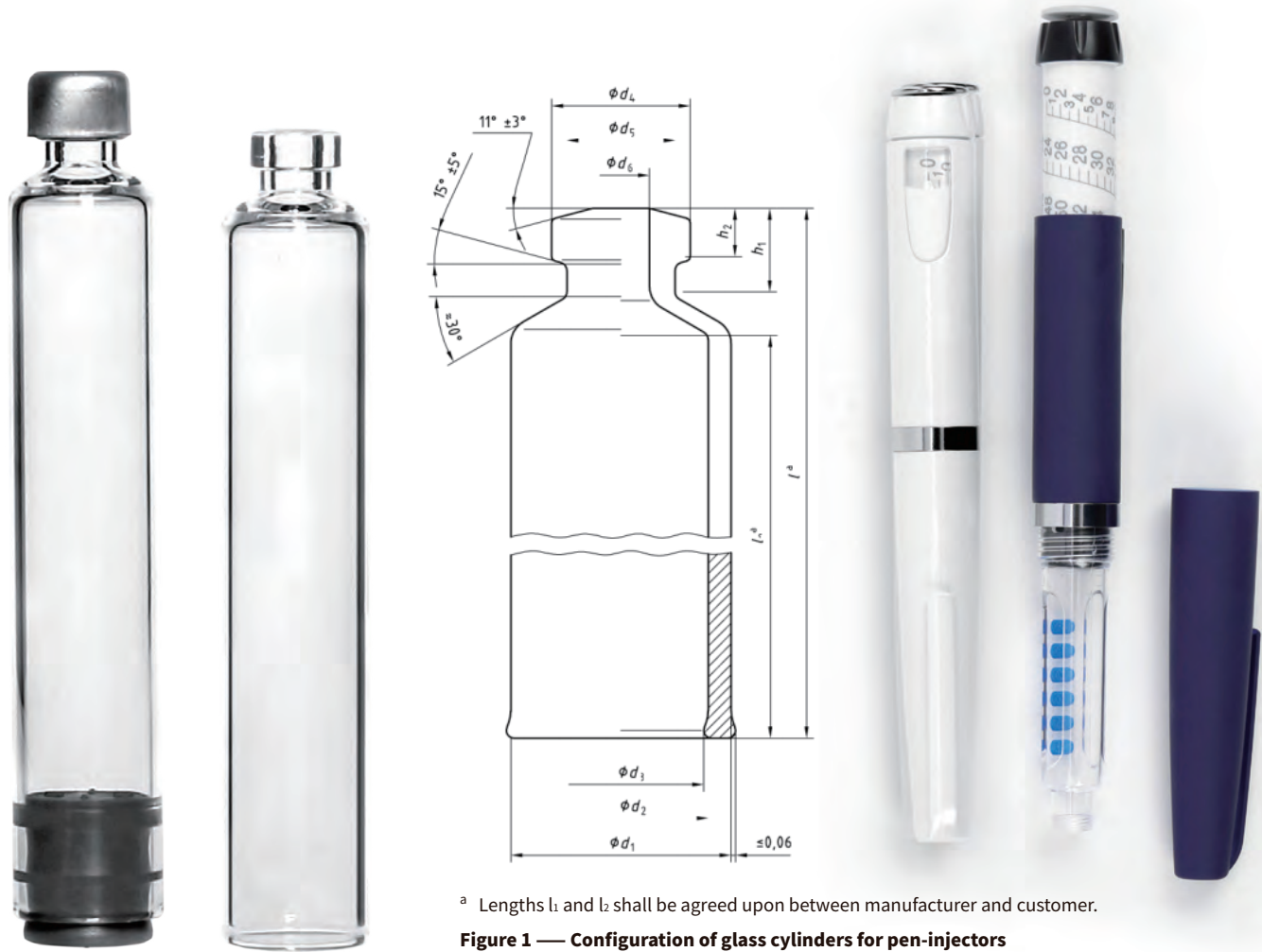
Figure 1 — Configuration of glass cylinders for pen-injectors
